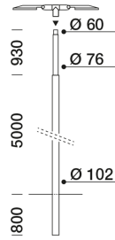
8650006 Ø 102/76 mm H. 6 m pole (Ø 60 mm connection) 0,8 m ground recessed
