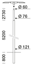
8650008 Ø 121/76 mm H. 8 m pole (Ø 60 mm connection) 0,8 m ground recessed
