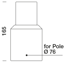
8650025 Ø 76 mm pole adaptor for single light fittings
