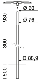
8650004 Ø 89/76 mm H. 4 m pole (Ø 60 mm connection) 0,5 m ground recessed
