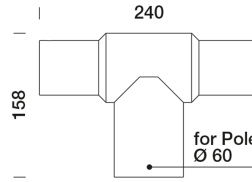
8650020 Ø 60 mm pole adaptor for two light fittings
