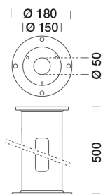
8950080 Recessed housing Ø 180 mm x D. 500 mm
